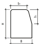
Randstein B 12 / 15 cm b_1 = 9 \text{ cm} / 12 \text{ cm} h_1 = 10 \text{ cm}
